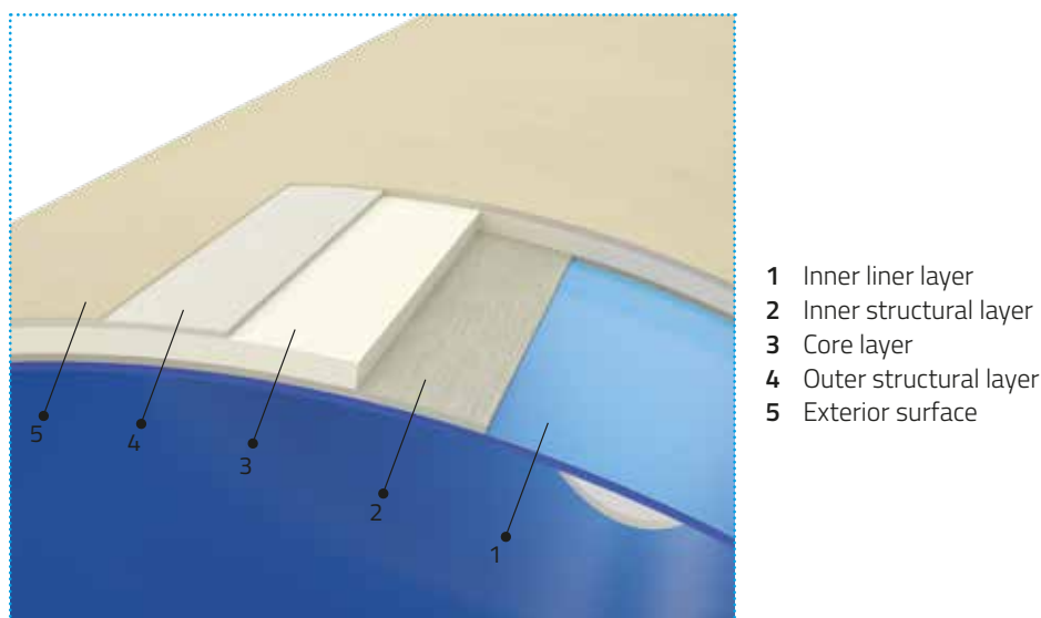
Wall structure of Amiblu NC Line pipe
