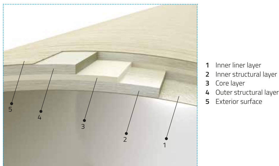
Wall structure of filament wound Amiblu pipe (Flowtite technology)
